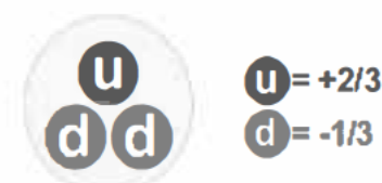
Figure 28.3 Neutron Quarks
