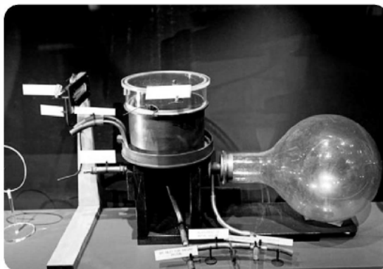
Figure 28.9 Wilson cloud Chambers
